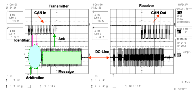
Figure 1 - Arbitration process over power line.
