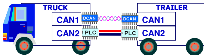
Figure 1.0 - Truck-Trailer Redundant communication
