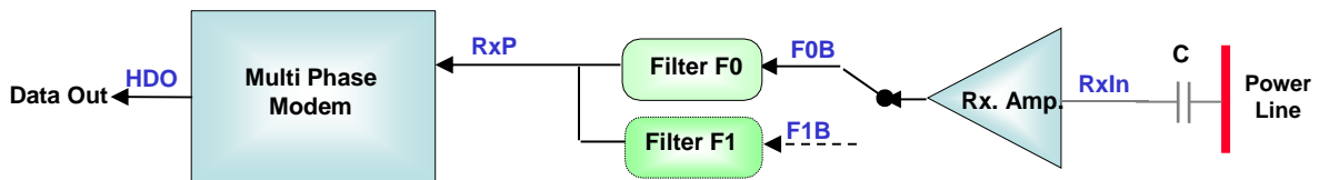
Figure 4.02 - Receive path.
